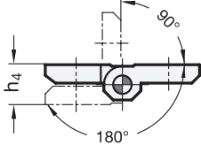
Swivelling range
