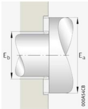
Mounting dimensions/raceway dimensions for direct bearing arrangement
