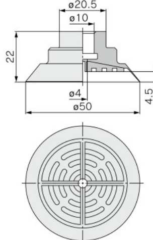
ZP3P-50PTSF [質量: 12.4g]
