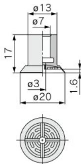
ZP3P-35PTSF [質量: 4.7g]
