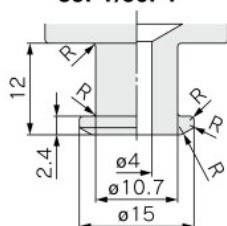
適応パッド 35PT/50PT
