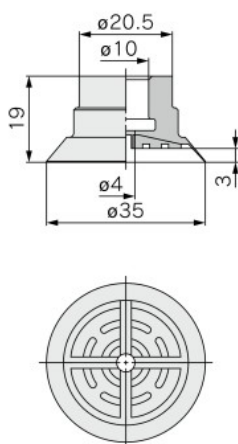
ZP3P-35PTSF [質量: 4.7g]
