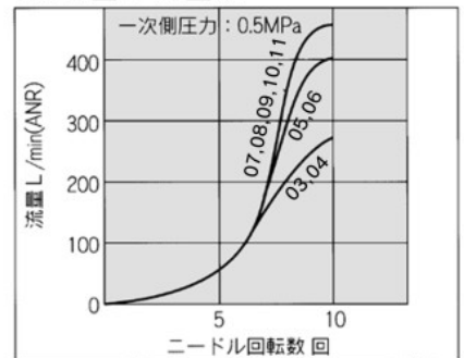
AS22□1FG-□02 AS23□1FG-□02
