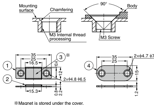
MC-YN015SP (Magnetic catch, counter plate and screws)
