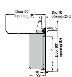
AZ-GD400-HL
