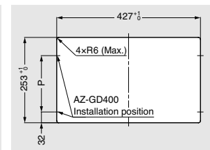
AZ-GD400-HL
