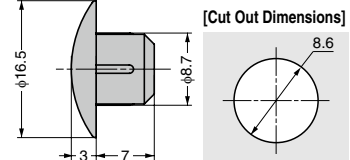
[Cut Out Dimensions]
