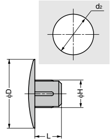
[Cut Out Dimensions]
